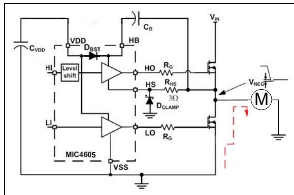
FIGURE 7-4: Negative HS Pin Voltage.
